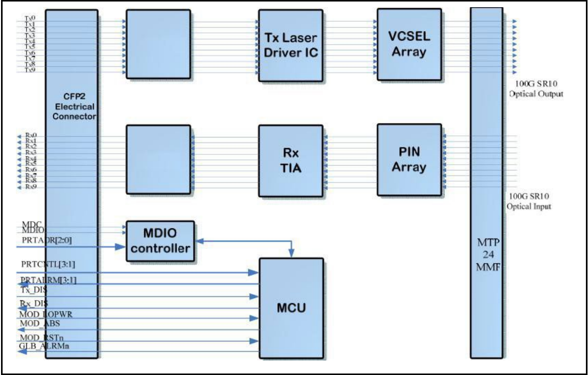
Functional Diagram
